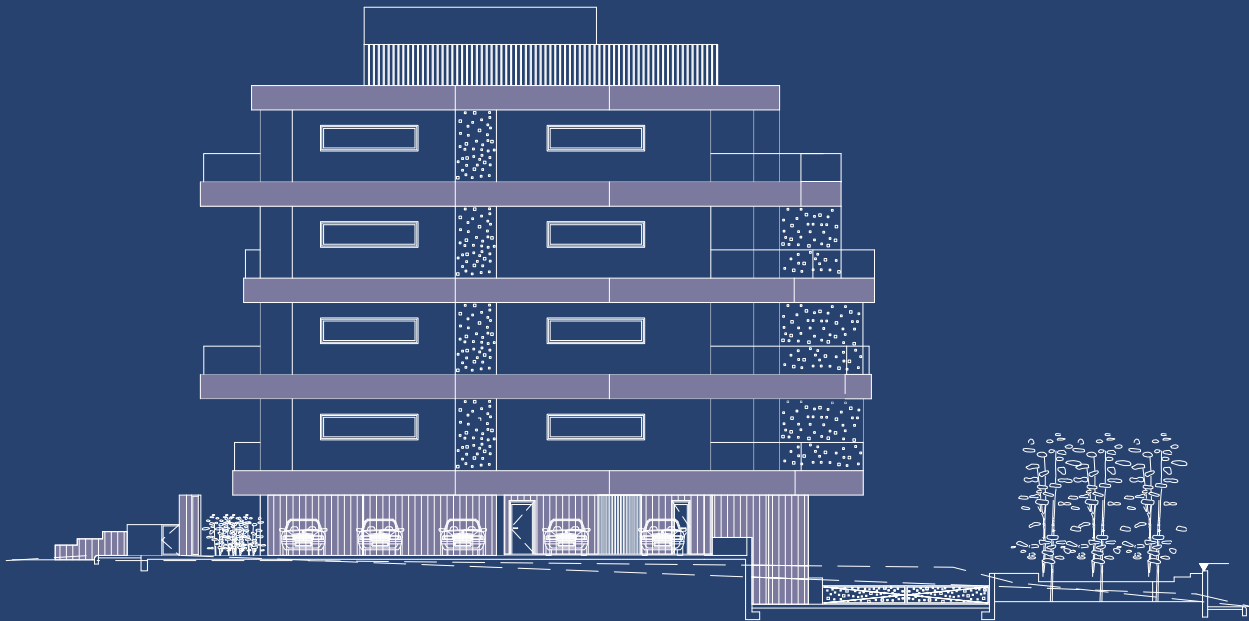
West Elevation
