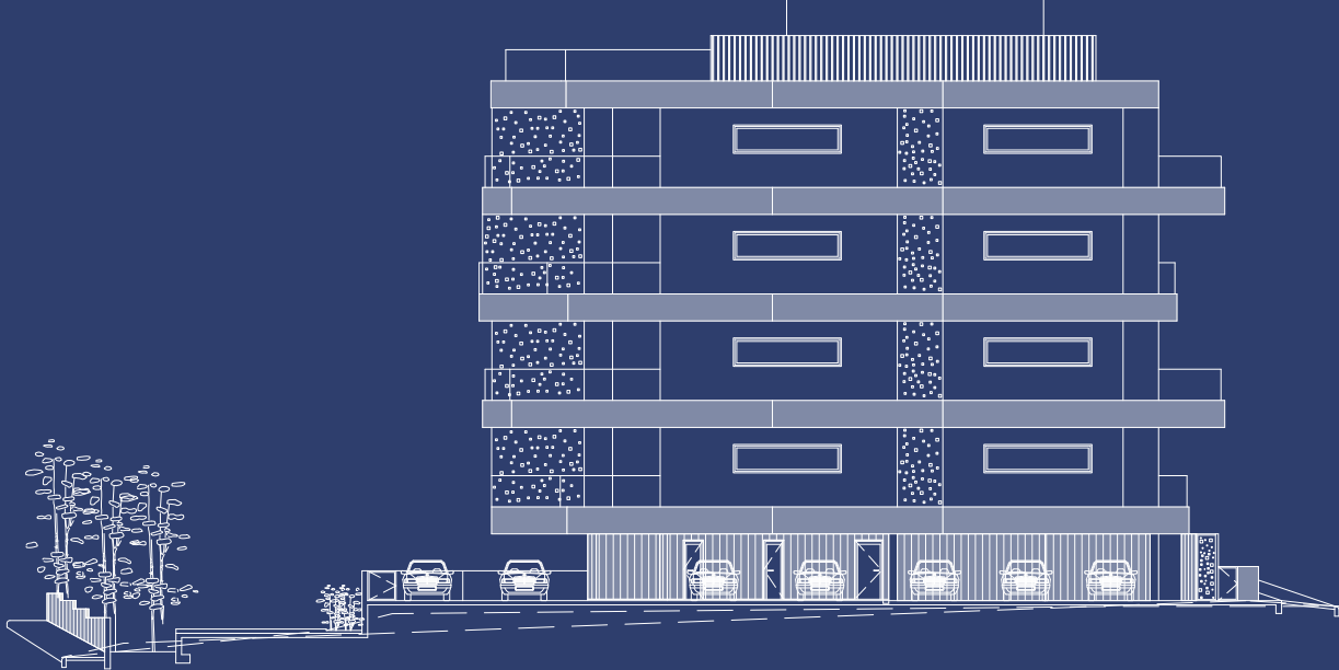
East Elevation
